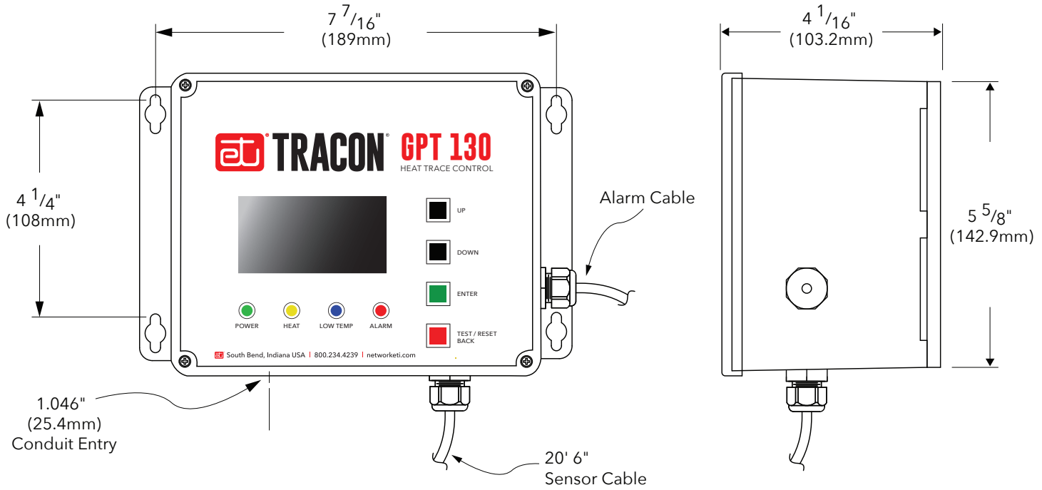
FIGURE 2. Mounting dimensions.
