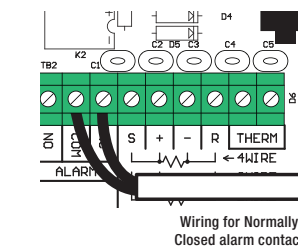
Figure 5. External alarm connection
